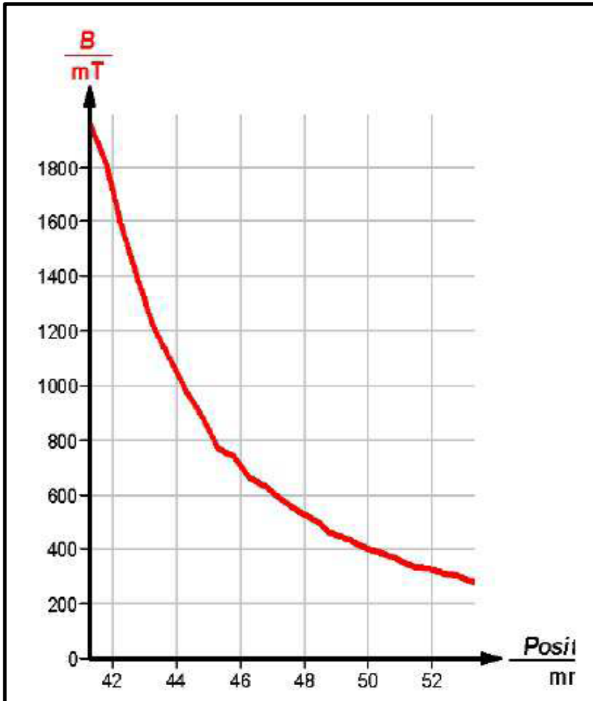
Fig. 3 Magnetic flux density B in the center of the gap without Cd lamp as a function of the shoe pole distance (without shoe pole tips)
