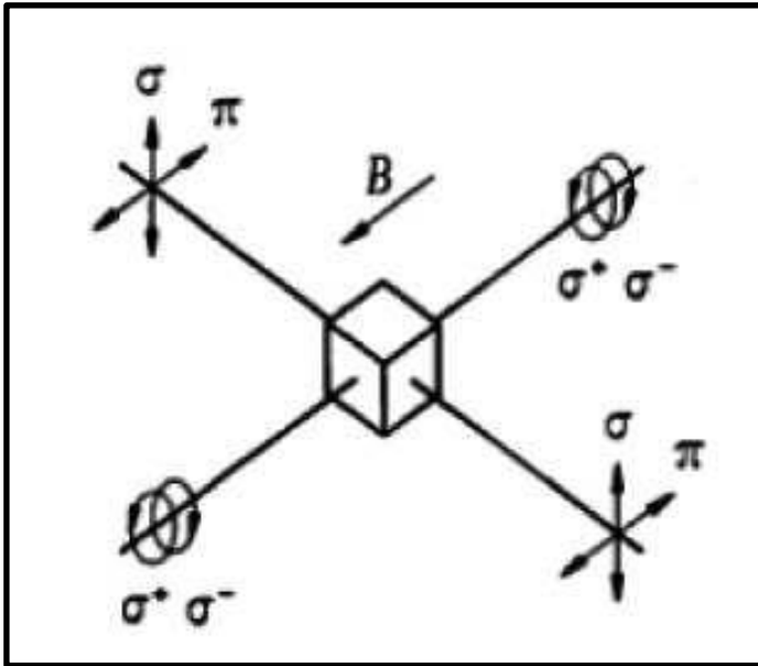
Fig. 5: Longitudinal and transversal Zeeman effect.
