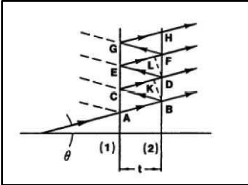
Fig. 8: Reflected and transmitted rays at the parallel surfaces (1) and (2) of the etalon. The etalon spacing is t = 3 \text{ mm} .
