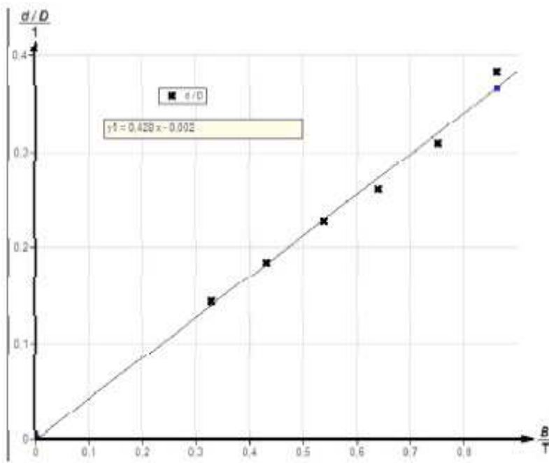
Fig. 15: Measurement results for \delta/\Delta vs. magnetic field strength.
