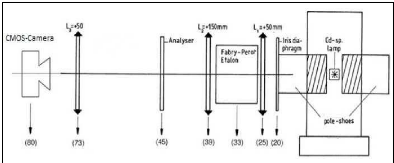
Fig. 2 Arrangements of the optical components.
