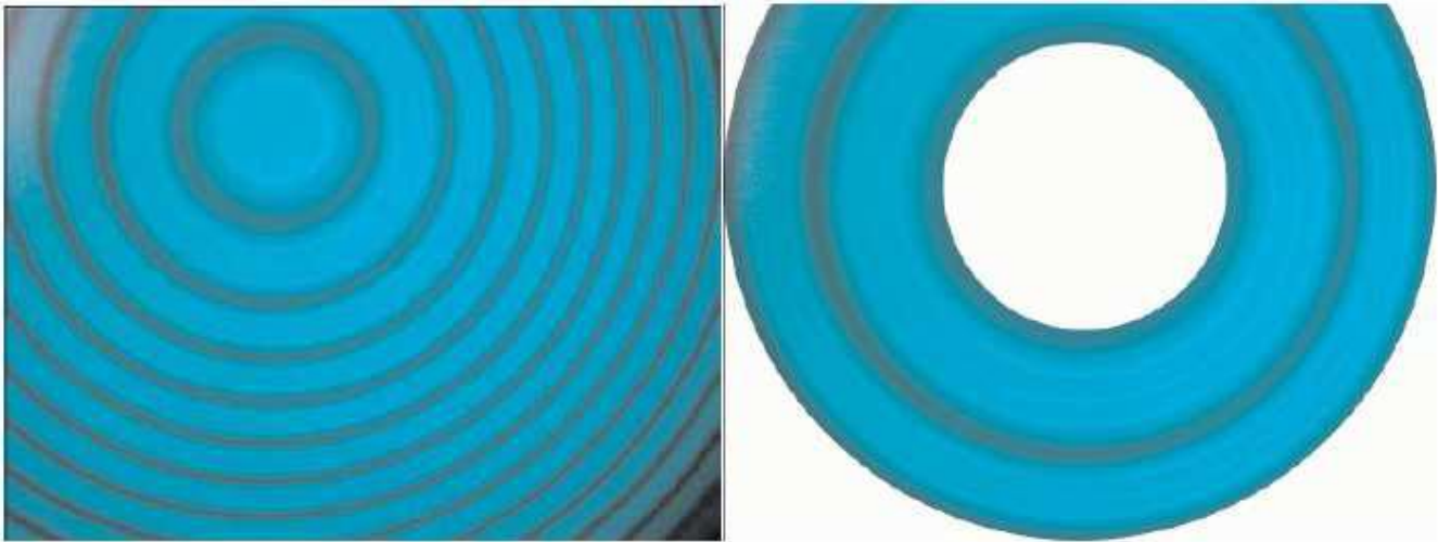
Fig. 11: Anomalous Zeeman effect: Interference pattern without polarization filter and magnified cut-out of the first completely visible two orders of interference.
