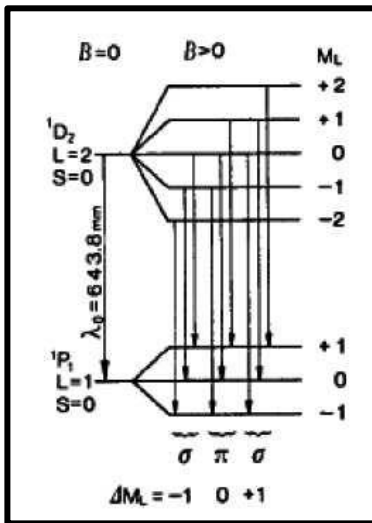
Fig. 6: Energy shift of the atomic states.
