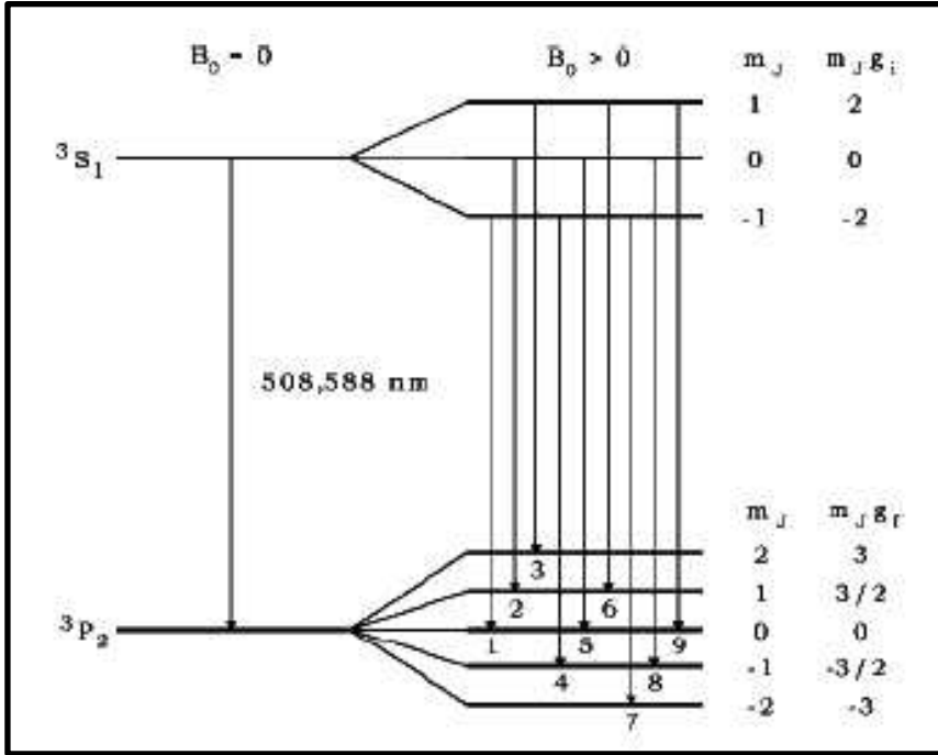
Fig. 7: Energy shift of the atomic states
